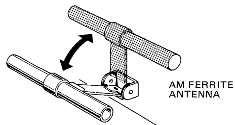
Fig. 6 — Adjust AM broadcast reception with this AM ferrite bar antenna.
