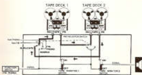
Fig. 13 - Tape duplicating: With the SX-7730 REC SELECTOR switch to DUPLICATE, tape duplicating can be performed by two units of tape deck: for example, first tape deck 1 (for playback) plays back signal, which is recorded by tape deck 2 (for recording) while causing the signal to flow in the arrow-indicated (→) direction.
