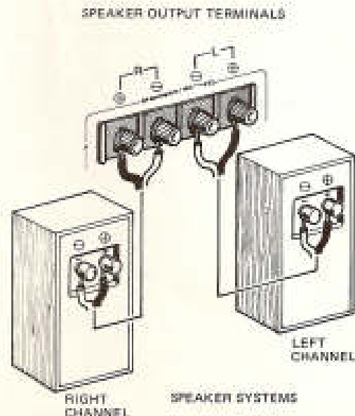
Fig. 2 - Connecting speaker output terminals of the SX-7730 to speaker systems.
