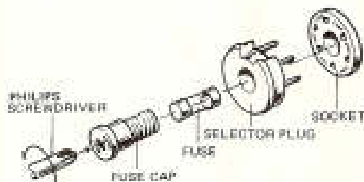
Take off the fuse cap by turning it with a philips screwdriver in the direction indicated by the arrow. Fig. B
