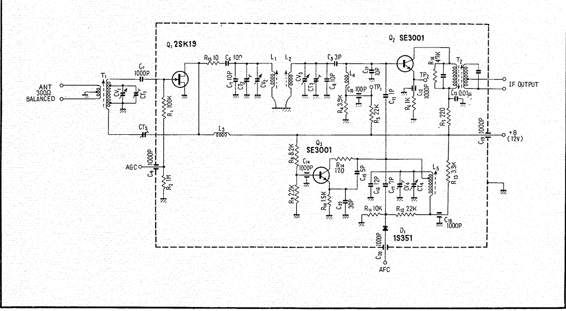
FM FRONT END W11-028
