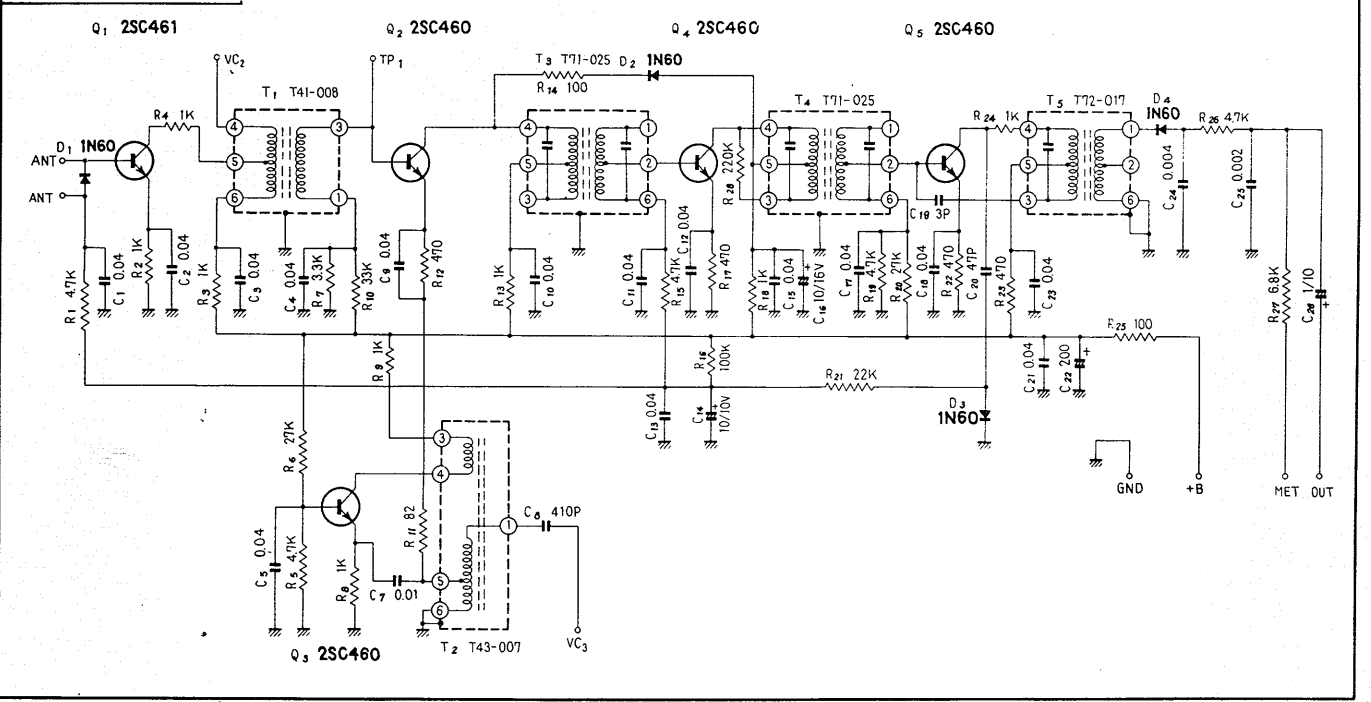
AM TUNER UNIT W14-008
